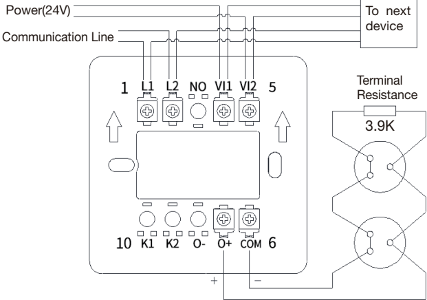
Figure 2: Wiring Diagram
