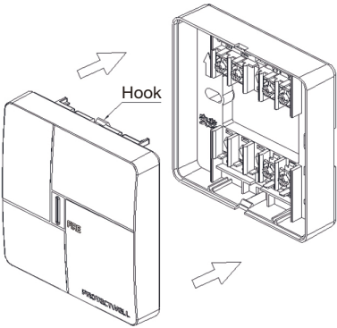
Figure 3: Mounting
