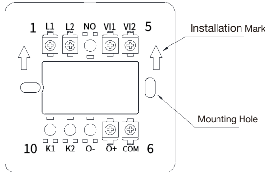
Figure 1: M600-6T Module Base
